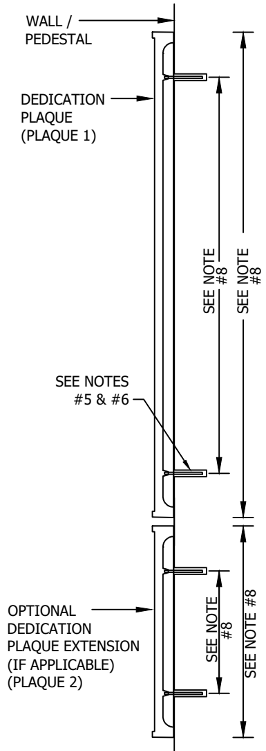
PLAQUE MOUNTING DETAIL
