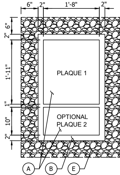
PLAN VIEW
