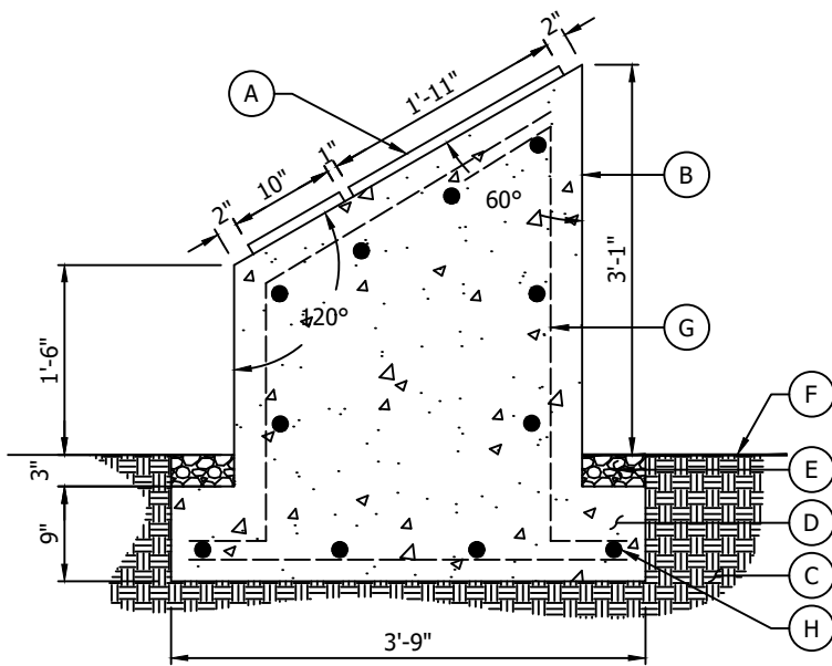
SIDE ELEVATION
