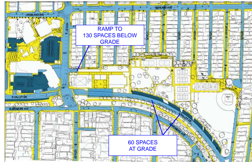
Live Oak Park Illustrative Vehicular Circulation and Parking Plan. Parking at Live Oak park is provided in two locations: sixty (60) spaces of at grade diagonal parking along the west side of Valley Drive and one hundred and thirty (130) spaces below grade underneath the library and community center accessed via a ramp at 15th street 120 feet west of Valley Drive. A vehicular drop-off/pick-up pedestrian court is provided on Valley Drive and service, delivering and loading for both the library and the community center in the below grade structure.
