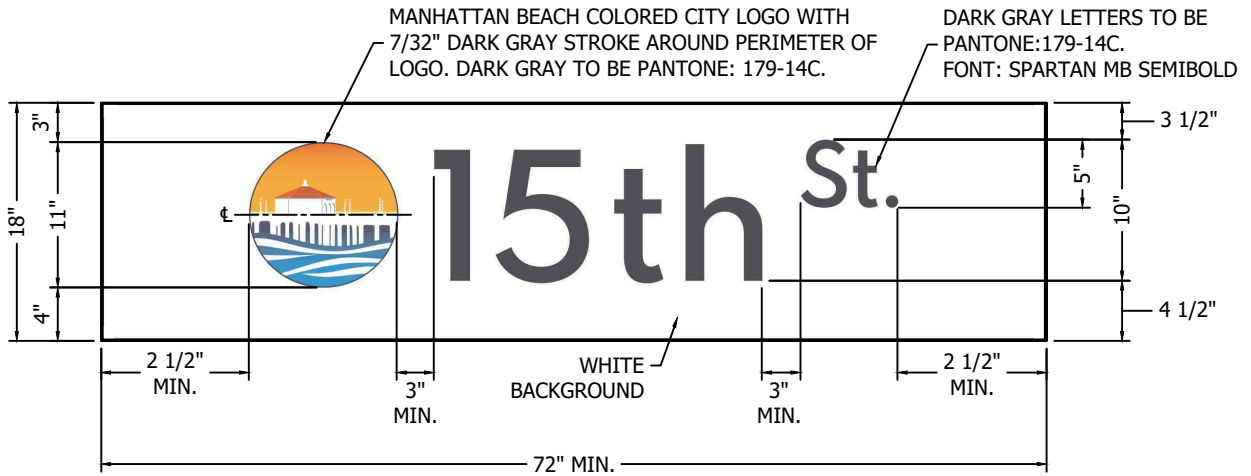
STANDARD INTERNALLY ILLUMINATED STREET NAME SIGN PANEL NOT TO SCALE
