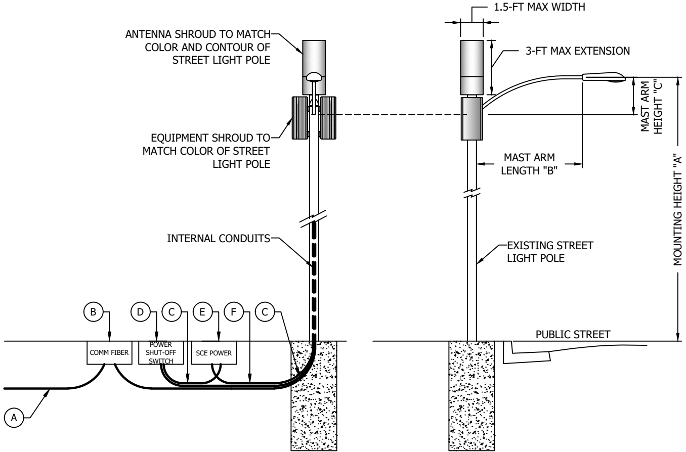
STREET-SIDE VIEW
